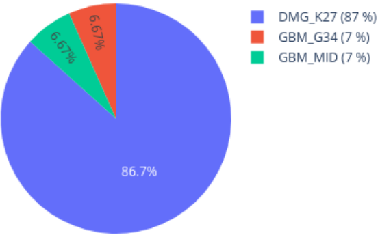
Neighbors in UMAP for 209808310041_R05C01 reference: AllIDATv2_20210804_HPAP_Sarc.xlsx (19967 cases), 0 CpGs
