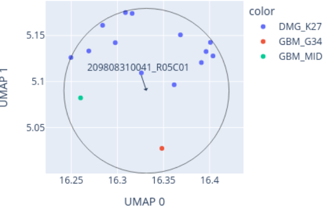
Close-up of UMAP for 209808310041_R05C01 reference: AllIDATv2_20210804_HPAP_Sarc.xlsx (19967 cases), 0 CpGs
