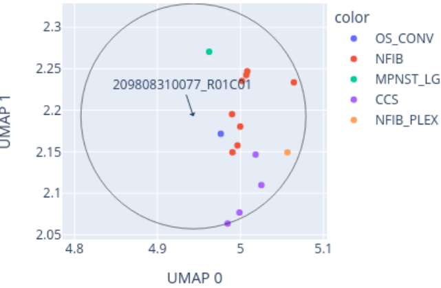
Close-up of UMAP for 209808310077_R01C01 reference: AllIDATv2_20210804_HPAP_Sarc.xlsx (19967 cases), 0 CpGs
