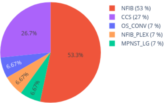
Neighbors in UMAP for 209808310077_R01C01 reference: AllIDATv2_20210804_HPAP_Sarc.xlsx (19967 cases), 0 CpGs
