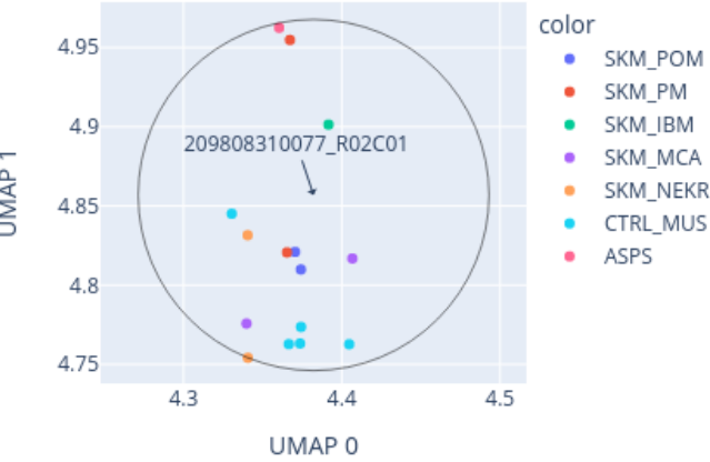
Close-up of UMAP for 209808310077_R02C01 reference: AllIDATv2_20210804_HPAP_Sarc.xlsx (19967 cases), 0 CpGs
