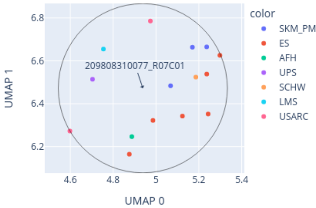
Close-up of UMAP for 209808310077_R07C01 reference: AllIDATv2_20210804_HPAP_Sarc.xlsx (19967 cases), 0 CpGs
