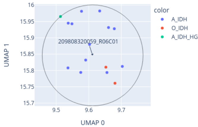
Close-up of UMAP for 209808320059_R06C01 reference: AllIDATv2_20210804_HPAP_Sarc.xlsx (19967 cases), 0 CpGs
