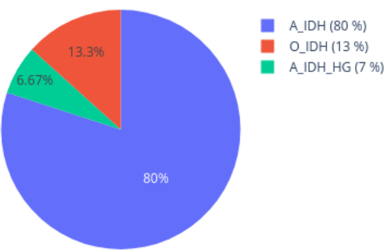
Neighbors in UMAP for 209808320059_R06C01 reference: AllIDATv2_20210804_HPAP_Sarc.xlsx (19967 cases), 0 CpGs
