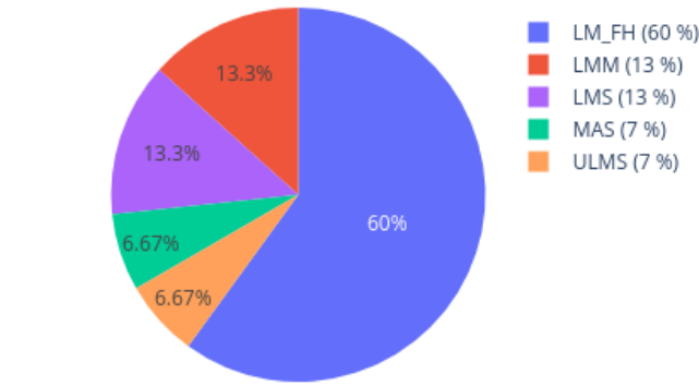
Neighbors in UMAP for 209808320082_R08C01 reference: EpiDip_BTRC_20250105.xlsx (3684 cases), 0 CpGs
