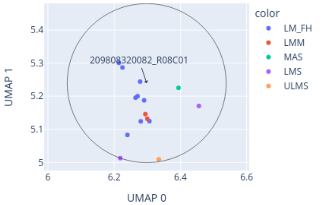
Close-up of UMAP for 209808320082_R08C01 reference: EpiDip_BTRC_20250105.xlsx (3684 cases), 0 CpGs
