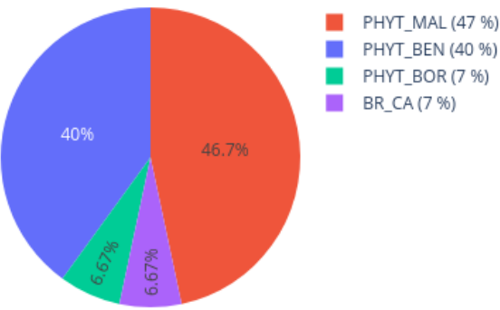
Neighbors in UMAP for 209808320170_R01C01 reference: AllIDATv2_20210804_HPAP_Sarc.xlsx (19967 cases), 0 CpGs
