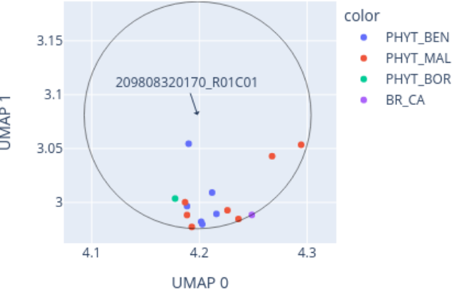
Close-up of UMAP for 209808320170_R01C01 reference: AllIDATv2_20210804_HPAP_Sarc.xlsx (19967 cases), 0 CpGs
