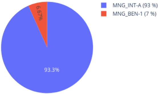
Neighbors in UMAP for 209815480053_R07C01 reference: AllIDATv2_20210804_HPAP_Sarc.xlsx (19967 cases), 0 CpGs
