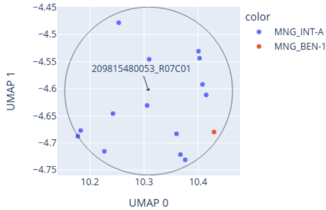
Close-up of UMAP for 209815480053_R07C01 reference: AllIDATv2_20210804_HPAP_Sarc.xlsx (19967 cases), 0 CpGs
