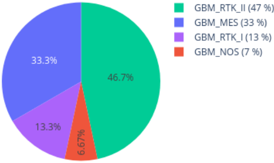
Neighbors in UMAP for 209815480053_R08C01 reference: AllIDATv2_20210804_HPAP_Sarc.xlsx (19967 cases), 0 CpGs
