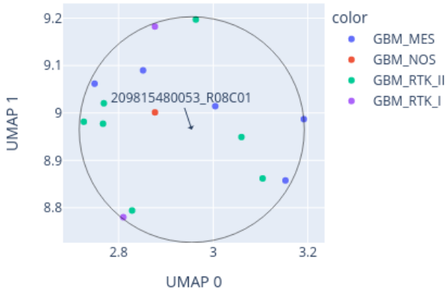
Close-up of UMAP for 209815480053_R08C01 reference: AllIDATv2_20210804_HPAP_Sarc.xlsx (19967 cases), 0 CpGs
