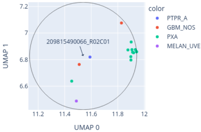
Close-up of UMAP for 209815490066_R02C01 reference: AllIDATv2_20210804_HPAP_Sarc.xlsx (19967 cases), 0 CpGs
