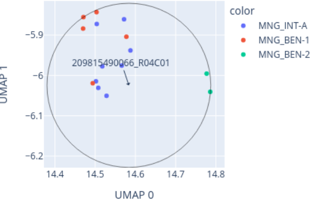
Close-up of UMAP for 209815490066_R04C01 reference: MNG_lfp_v1.xlsx (705 cases), 0 CpGs
