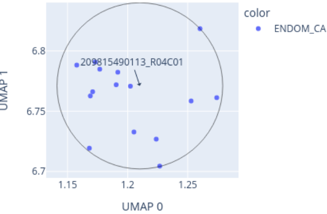
Close-up of UMAP for 209815490113_R04C01 reference: AllIDATv2_20210804_HPAP_Sarc.xlsx (19967 cases), 0 CpGs
