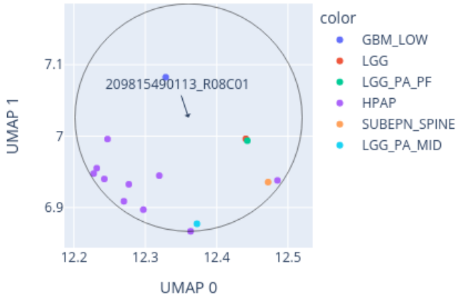
Close-up of UMAP for 209815490113_R08C01 reference: AllIDATv2_20210804_HPAP_Sarc.xlsx (19967 cases), 0 CpGs
