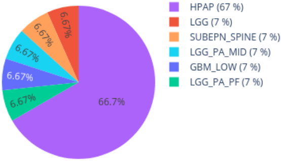
Neighbors in UMAP for 209815490113_R08C01 reference: AllIDATv2_20210804_HPAP_Sarc.xlsx (19967 cases), 0 CpGs
