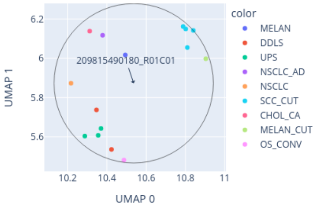
Close-up of UMAP for 209815490180_R01C01 reference: AllIDATv2_20210804_HPAP_Sarc.xlsx (19967 cases), 0 CpGs
