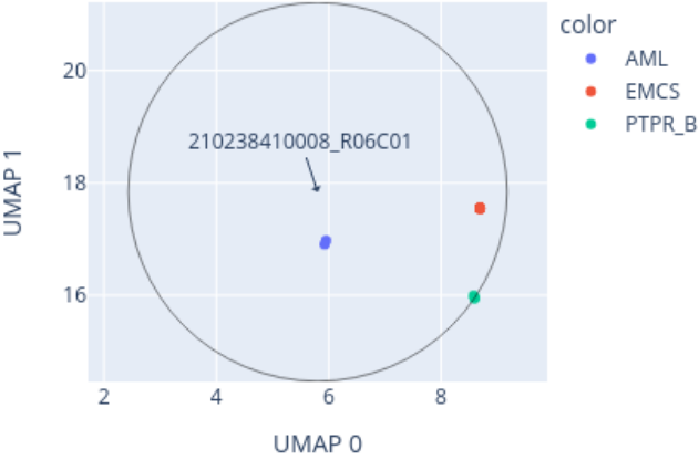
Close-up of UMAP for 210238410008_R06C01 reference: AllIDATv2_20210804_HPAP_Sarc.xlsx (19967 cases), 0 CpGs
