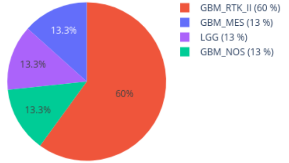
Neighbors in UMAP for 210246750011_R05C01 reference: AllIDATv2_20210804_HPAP_Sarc.xlsx (19967 cases), 0 CpGs
