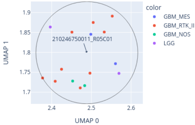
Close-up of UMAP for 210246750011_R05C01 reference: AllIDATv2_20210804_HPAP_Sarc.xlsx (19967 cases), 0 CpGs
