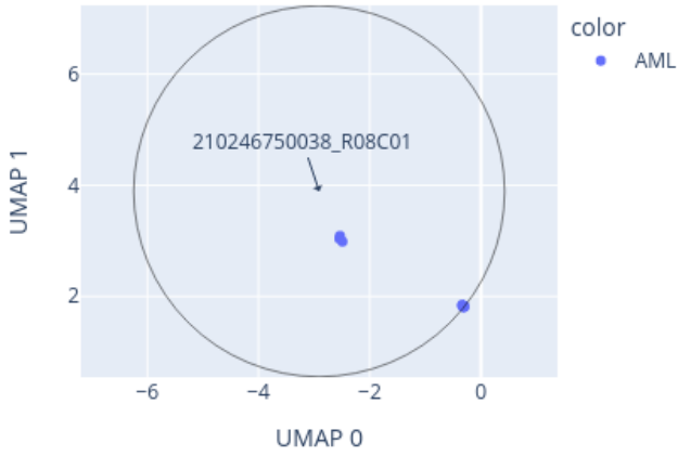
Close-up of UMAP for 210246750038_R08C01 reference: AllIDATv2_20210804_HPAP_Sarc.xlsx (19967 cases), 0 CpGs
