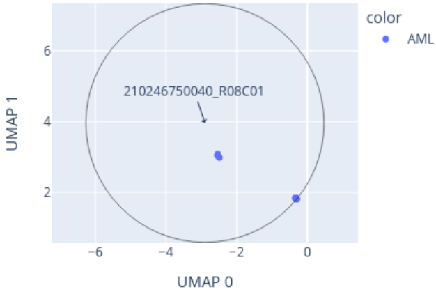
Close-up of UMAP for 210246750040_R08C01 reference: AllIDATv2_20210804_HPAP_Sarc.xlsx (19967 cases), 0 CpGs
