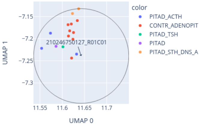
Close-up of UMAP for 210246750127_R01C01 reference: AllIDATv2_20210804_HPAP_Sarc.xlsx (19967 cases), 0 CpGs
