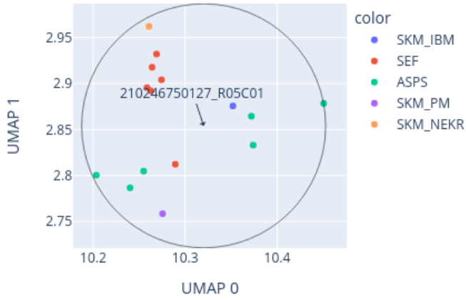
Close-up of UMAP for 210246750127_R05C01 reference: AllIDATv2_20210804_HPAP_Sarc.xlsx (19967 cases), 0 CpGs
