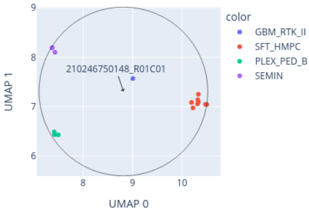
Close-up of UMAP for 210246750148_R01C01 reference: GSE90496_lfp02.xlsx (2980 cases), 0 CpGs
