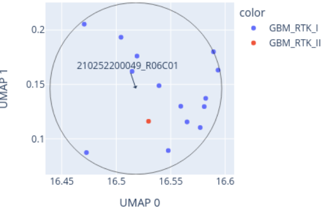
Close-up of UMAP for 210252200049_R06C01 reference: AllIDATv2_20210804_HPAP_Sarc.xlsx (19967 cases), 0 CpGs
