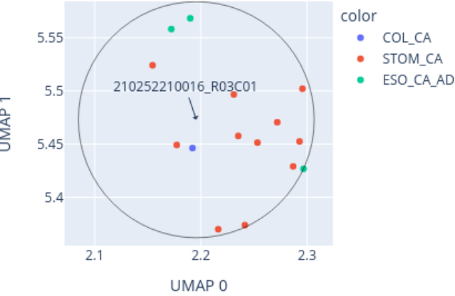
Close-up of UMAP for 210252210016_R03C01 reference: AllIDATv2_20210804_HPAP_Sarc.xlsx (19967 cases), 0 CpGs
