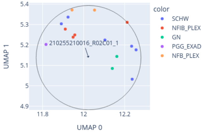
Close-up of UMAP for 210255210016_R02C01_1 reference: AllIDATv2_20210804_HPAP_Sarc.xlsx (19967 cases), 0 CpGs
