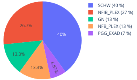
Neighbors in UMAP for 210255210016_R02C01_1 reference: AllIDATv2_20210804_HPAP_Sarc.xlsx (19967 cases), 0 CpGs
