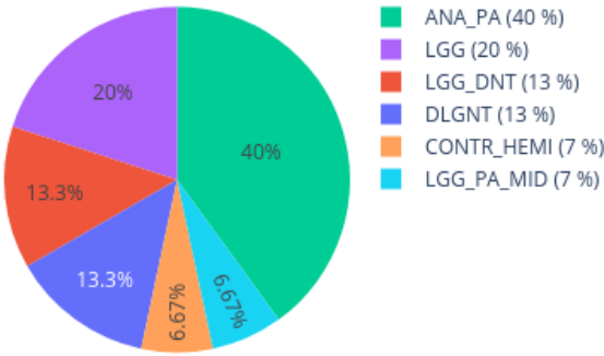
Neighbors in UMAP for 210255900031_R02C01 reference: AllIDATv2_20210804_HPAP_Sarc.xlsx (19967 cases), 0 CpGs
