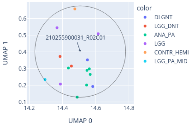
Close-up of UMAP for 210255900031_R02C01 reference: AllIDATv2_20210804_HPAP_Sarc.xlsx (19967 cases), 0 CpGs
