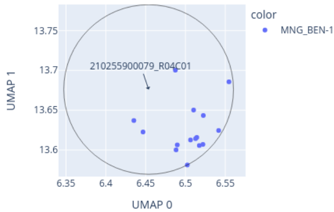
Close-up of UMAP for 210255900079_R04C01 reference: AllIDATv2_20210804_HPAP_Sarc.xlsx (19967 cases), 0 CpGs
