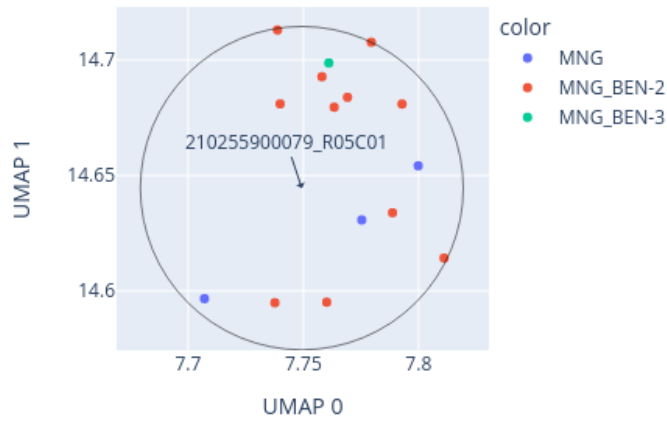
Close-up of UMAP for 210255900079_R05C01 reference: AllIDATv2_20210804_HPAP_Sarc.xlsx (19967 cases), 0 CpGs
