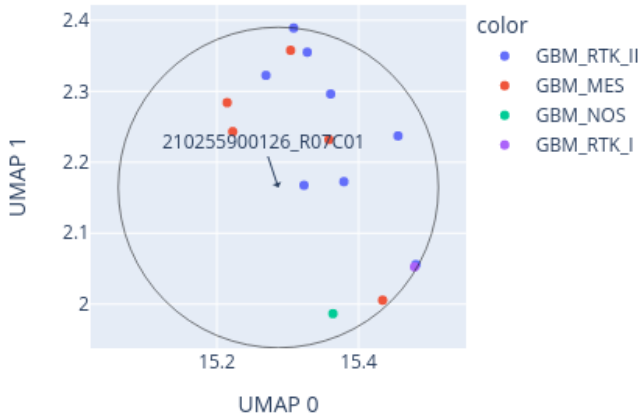
Close-up of UMAP for 210255900126_R07C01 reference: AllIDATv2_20210804_HPAP_Sarc.xlsx (19967 cases), 0 CpGs
