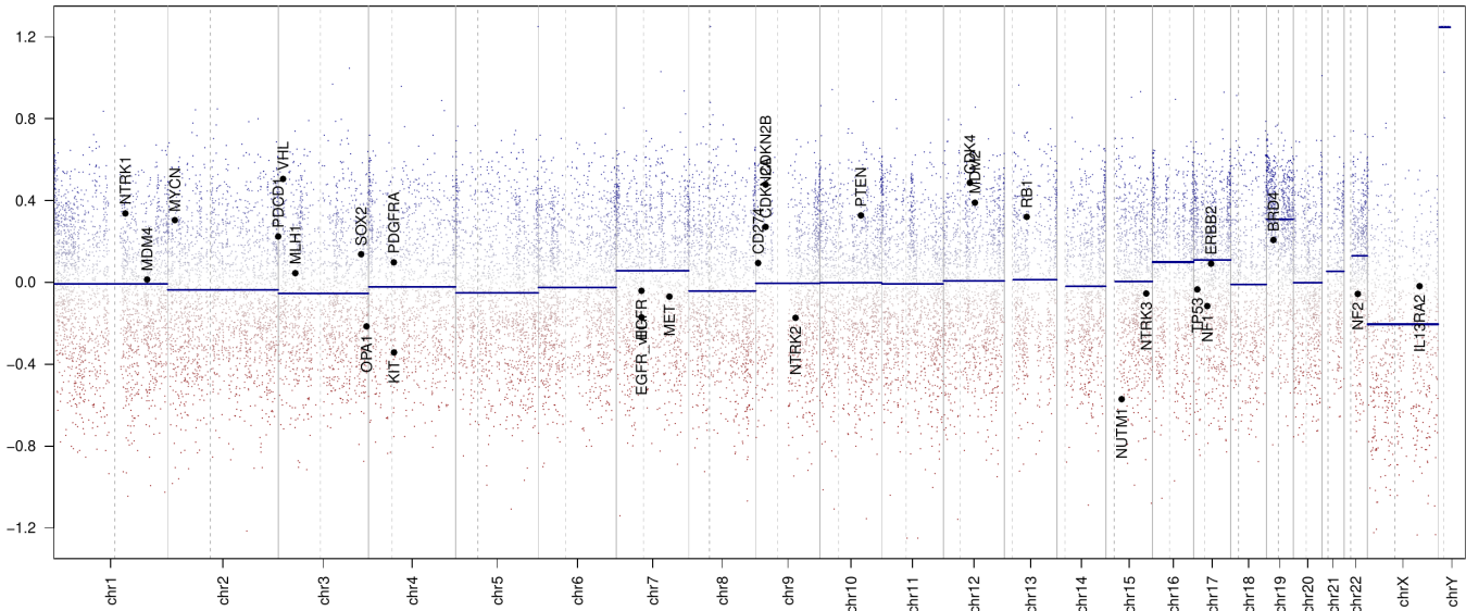
210255900174_R01C01
