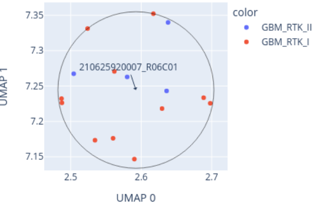
Close-up of UMAP for 210625920007_R06C01 reference: AllIDATv2_20210804_HPAP_Sarc.xlsx (19967 cases), 0 CpGs
