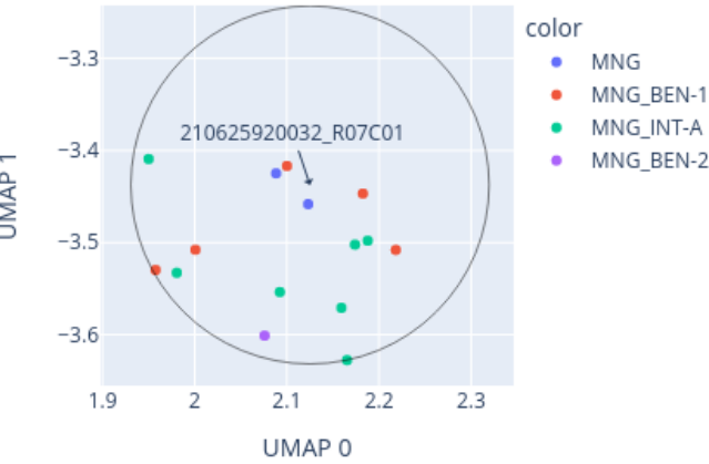
Close-up of UMAP for 210625920032_R07C01 reference: AllIDATv2_20210804_HPAP_Sarc.xlsx (19967 cases), 0 CpGs
