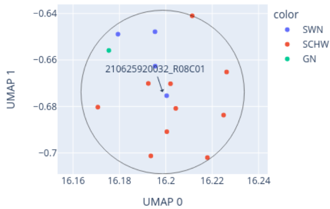
Close-up of UMAP for 210625920032_R08C01 reference: AllIDATv2_20210804_HPAP_Sarc.xlsx (19967 cases), 0 CpGs
