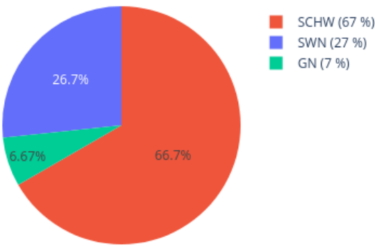
Neighbors in UMAP for 210625920032_R08C01 reference: AllIDATv2_20210804_HPAP_Sarc.xlsx (19967 cases), 0 CpGs
