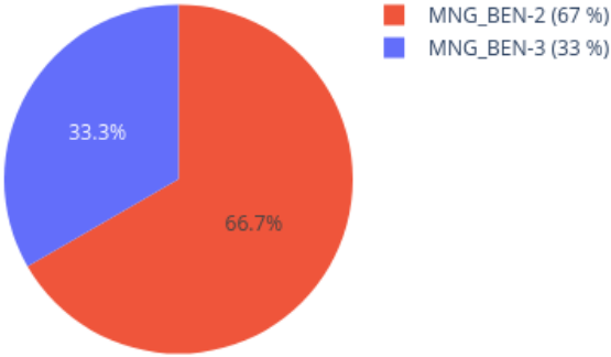
Neighbors in UMAP for 210625920033_R05C01 reference: AllIDATv2_20210804_HPAP_Sarc.xlsx (19967 cases), 0 CpGs
