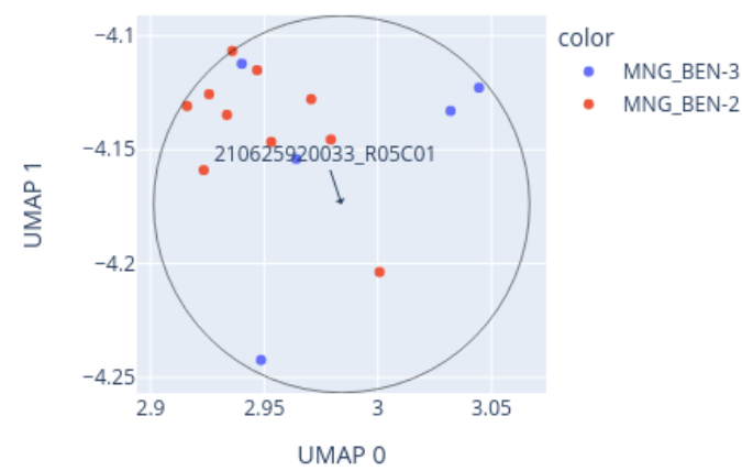
Close-up of UMAP for 210625920033_R05C01 reference: AllIDATv2_20210804_HPAP_Sarc.xlsx (19967 cases), 0 CpGs
