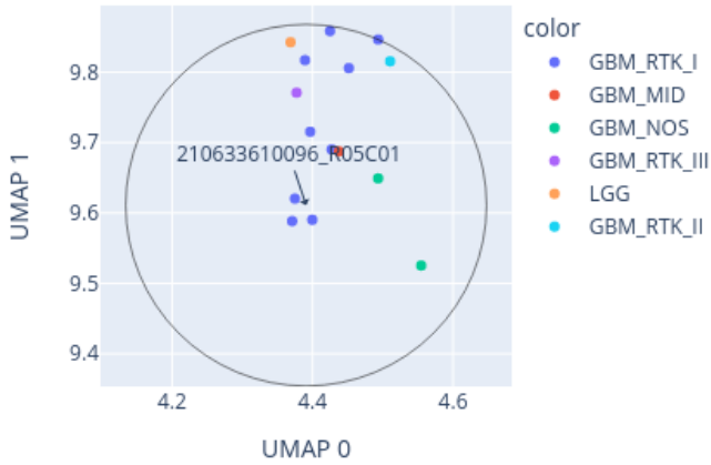
Close-up of UMAP for 210633610096_R05C01 reference: AllIDATv2_20210804_HPAP_Sarc.xlsx (19967 cases), 0 CpGs
