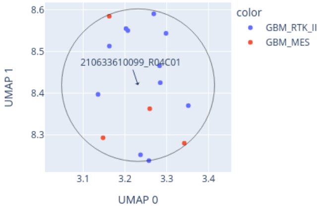
Close-up of UMAP for 210633610099_R04C01 reference: AllIDATv2_20210804_HPAP_Sarc.xlsx (19967 cases), 0 CpGs
