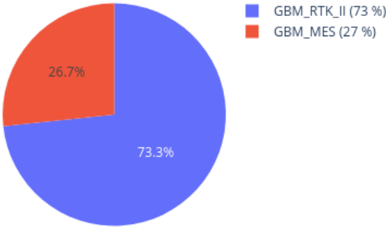
Neighbors in UMAP for 210633610099_R04C01 reference: AllIDATv2_20210804_HPAP_Sarc.xlsx (19967 cases), 0 CpGs
