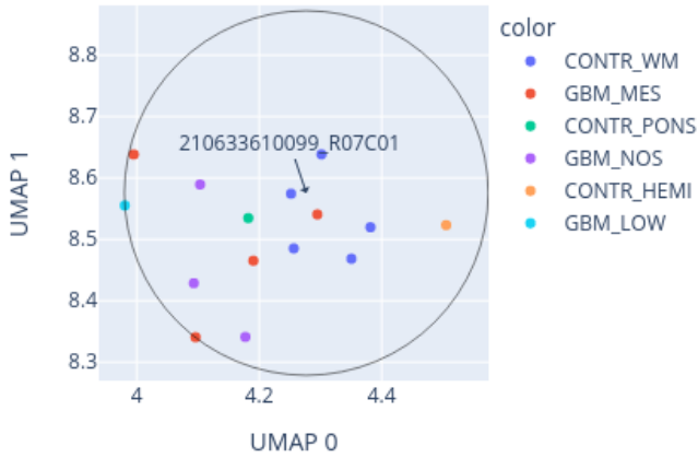
Close-up of UMAP for 210633610099_R07C01 reference: AllIDATv2_20210804_HPAP_Sarc.xlsx (19967 cases), 0 CpGs
