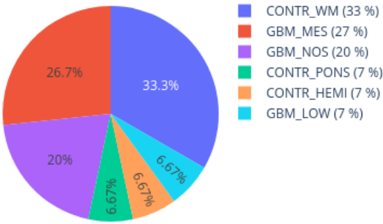
Neighbors in UMAP for 210633610099_R07C01 reference: AllIDATv2_20210804_HPAP_Sarc.xlsx (19967 cases), 0 CpGs
