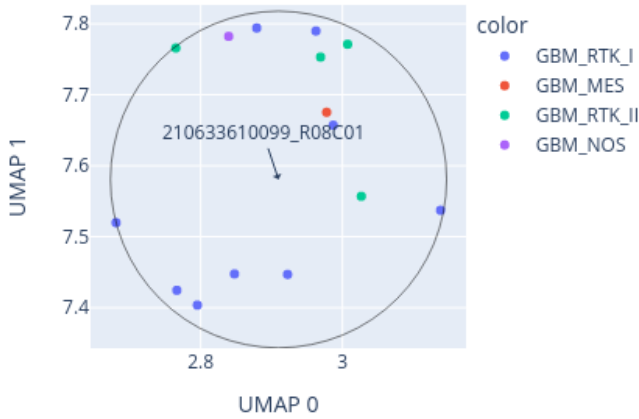
Close-up of UMAP for 210633610099_R08C01 reference: AllIDATv2_20210804_HPAP_Sarc.xlsx (19967 cases), 0 CpGs
