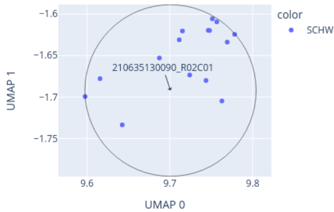
Close-up of UMAP for 210635130090_R02C01 reference: AllIDATv2_20210804_HPAP_Sarc.xlsx (19967 cases), 0 CpGs
