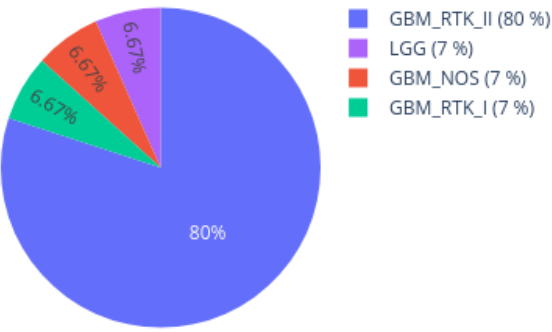
Neighbors in UMAP for 210635130093_R06C01 reference: AllIDATv2_20210804_HPAP_Sarc.xlsx (19967 cases), 0 CpGs
