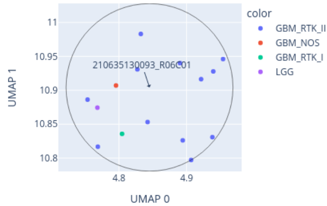
Close-up of UMAP for 210635130093_R06C01 reference: AllIDATv2_20210804_HPAP_Sarc.xlsx (19967 cases), 0 CpGs
