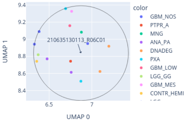
Close-up of UMAP for 210635130113_R06C01 reference: AllIDATv2_20210804_HPAP_Sarc.xlsx (19967 cases), 0 CpGs
