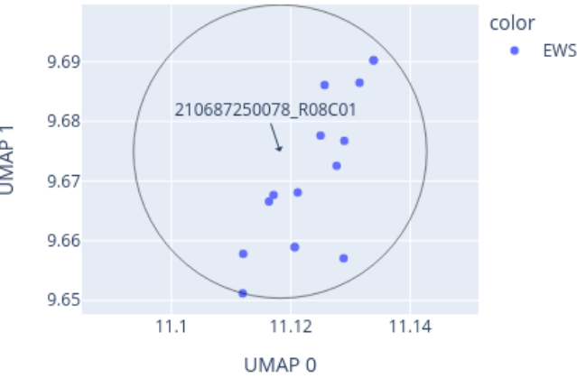
Close-up of UMAP for 210687250078_R08C01 reference: AllIDATv2_20210804_HPAP_Sarc.xlsx (19967 cases), 0 CpGs
