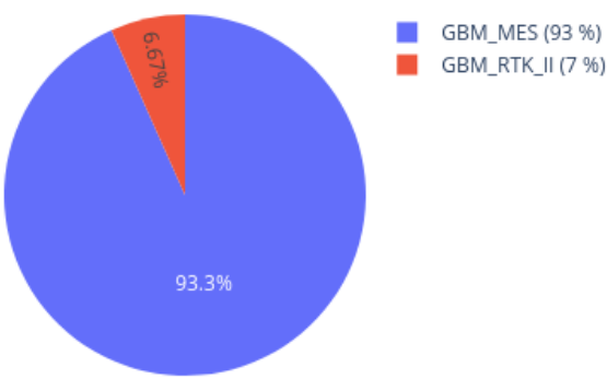
Neighbors in UMAP for 210687250100_R04C01 reference: AllIDATv2_20210804_HPAP_Sarc.xlsx (19967 cases), 0 CpGs
