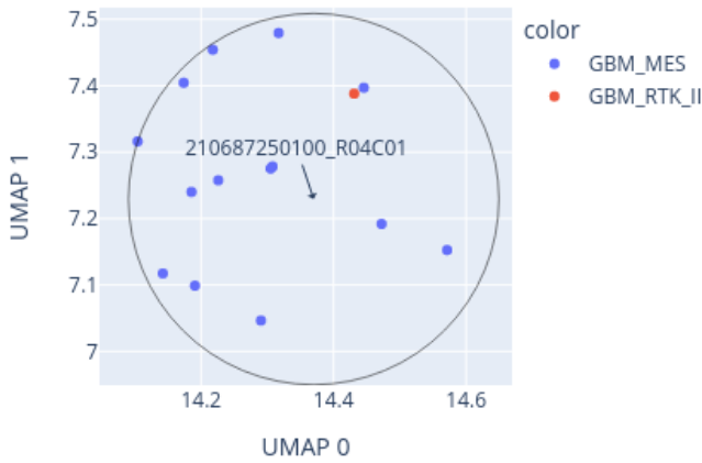
Close-up of UMAP for 210687250100_R04C01 reference: AllIDATv2_20210804_HPAP_Sarc.xlsx (19967 cases), 0 CpGs
