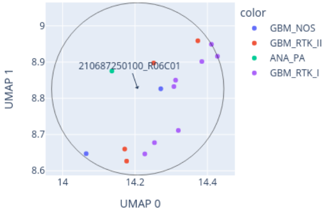
Close-up of UMAP for 210687250100_R06C01 reference: AllIDATv2_20210804_HPAP_Sarc.xlsx (19967 cases), 0 CpGs
