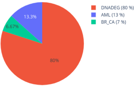
Neighbors in UMAP for 210687250102_R06C01 reference: AllIDATv2_20210804_HPAP_Sarc.xlsx (19967 cases), 0 CpGs
