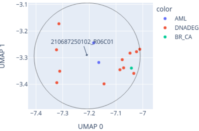
Close-up of UMAP for 210687250102_R06C01 reference: AllIDATv2_20210804_HPAP_Sarc.xlsx (19967 cases), 0 CpGs
