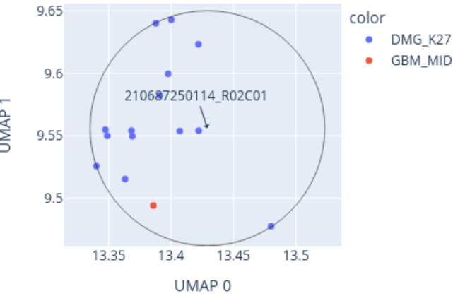
Close-up of UMAP for 210687250114_R02C01 reference: AllIDATv2_20210804_HPAP_Sarc.xlsx (19967 cases), 0 CpGs
