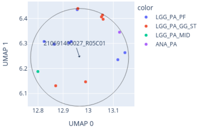
Close-up of UMAP for 210691400027_R05C01 reference: AllIDATv2_20210804_HPAP_Sarc.xlsx (19967 cases), 0 CpGs
