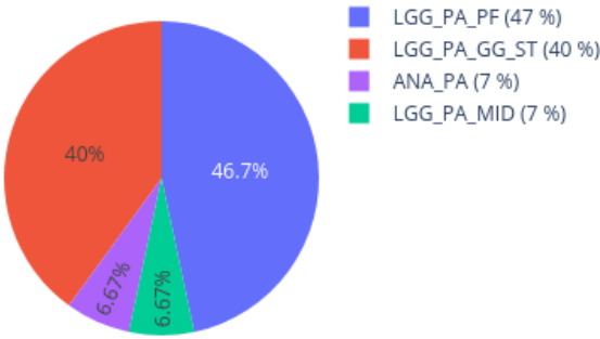
Neighbors in UMAP for 210691400027_R05C01 reference: AllIDATv2_20210804_HPAP_Sarc.xlsx (19967 cases), 0 CpGs
