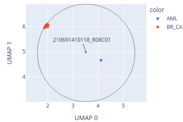
Close-up of UMAP for 210691410118_R08C01 reference: AllIDATv2_20210804_HPAP_Sarc.xlsx (19967 cases), 0 CpGs
