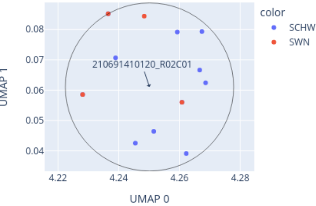
Close-up of UMAP for 210691410120_R02C01 reference: AllIDATv2_20210804_HPAP_Sarc.xlsx (19967 cases), 0 CpGs
