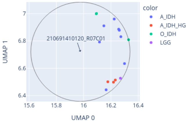
Close-up of UMAP for 210691410120_R07C01 reference: AllIDATv2_20210804_HPAP_Sarc.xlsx (19967 cases), 0 CpGs
