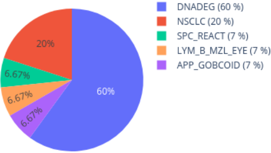
Neighbors in UMAP for 210696110080_R01C01 reference: AllIDATv2_20210804_HPAP_Sarc.xlsx (19967 cases), 0 CpGs
