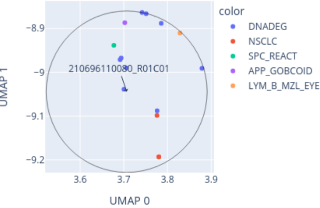
Close-up of UMAP for 210696110080_R01C01 reference: AllIDATv2_20210804_HPAP_Sarc.xlsx (19967 cases), 0 CpGs
